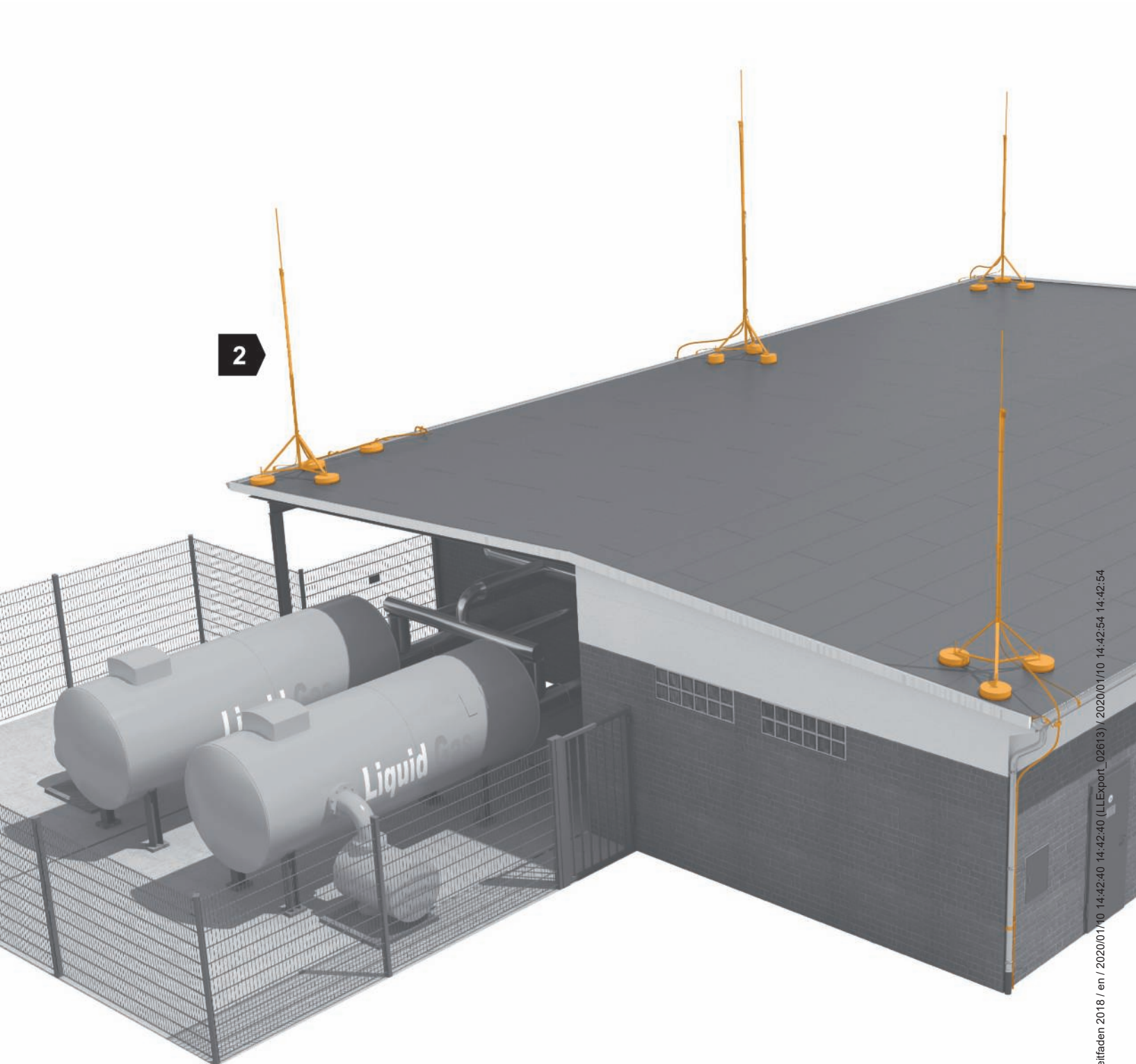
Installation principle for isCon® in potentially explosive areas
