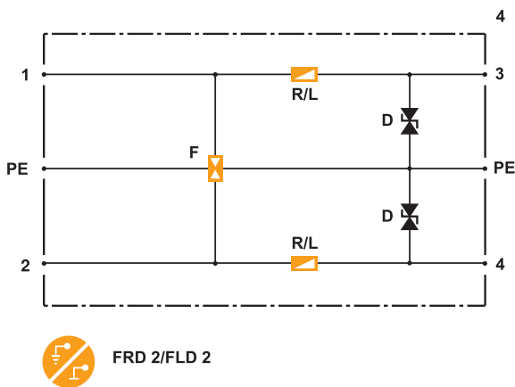
Circuit diagram of lightning barrier FRD2/FLD2
